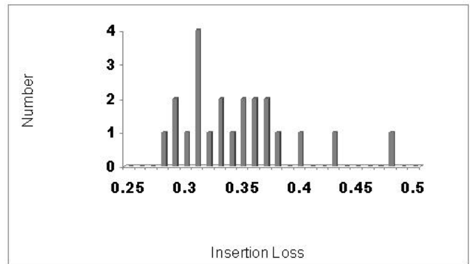
Fig. 8 Statistic diagram: Insertion Loss of Com-Ref port
