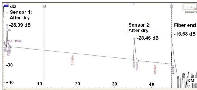
Fig. 4 OTDR traces after water sensor dried
