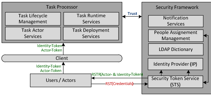
Figure 4. Overall architecture.
