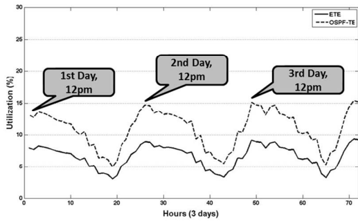
Figure 3. Link utilization when ETE and OSPF-TE are applied.
