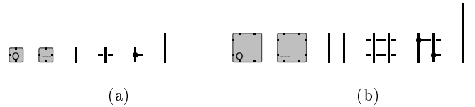
Fig. 11. Parameters d , d2 , w1 , w2 , w3 and w4 for (a) 1-bit, and (b) 2-bit computations
