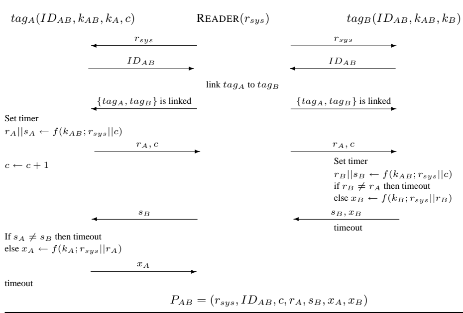
Fig. 1. A robust grouping-proof—for two tags
